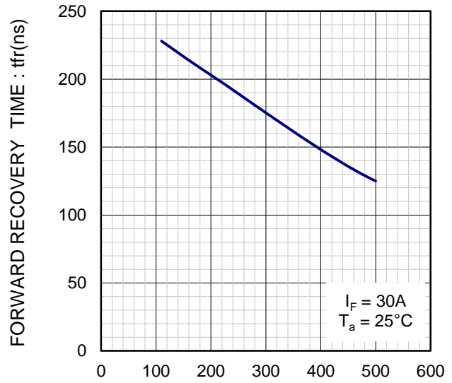
RATE OF CHANGE OF CURRENT : di/dt(A/μs) di/dt-t fr CHARACTERISTICS
