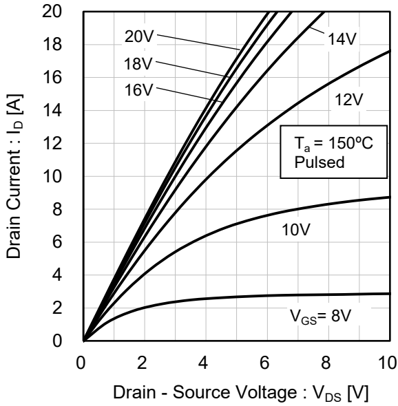
Fig.7 T_j = 150^\circ\text{C} Typical Output Characteristics(I)
