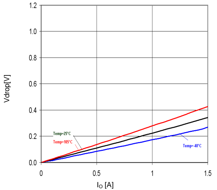
Figure 38. Minimum dropout Voltage 2 (V CC =12V, T a =25°C)
