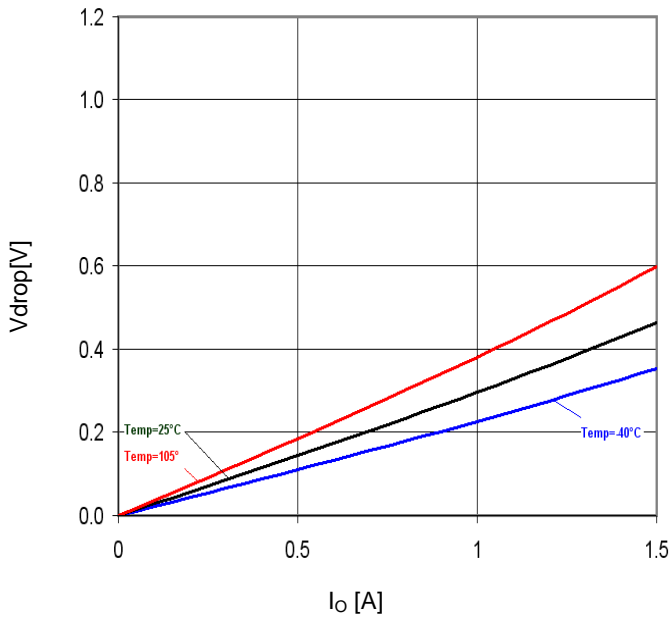
Figure 35. Minimum dropout Voltage 2 (V CC =6V, T a =25°C)
