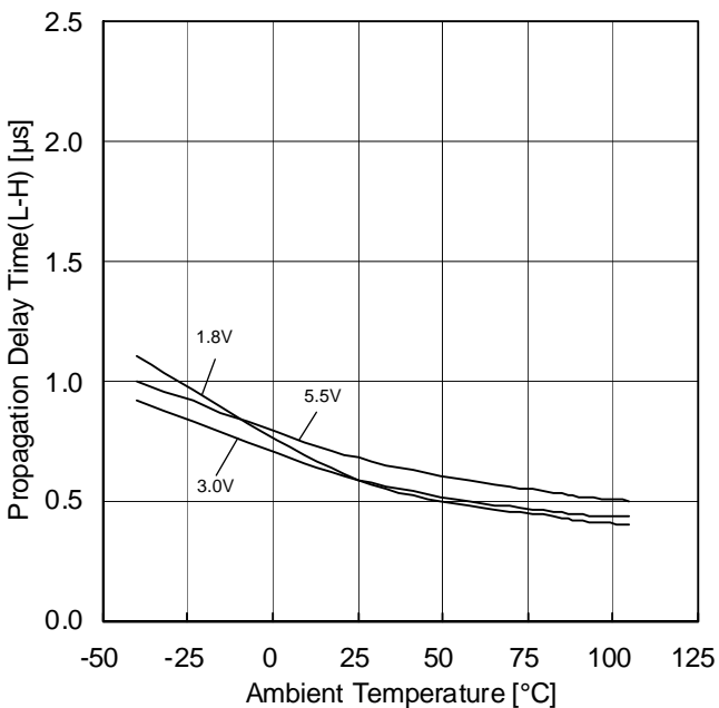
Figure 19. 立ち上がり伝播遅延(L-H)-温度特性 (R L =10kΩ, V RL =3V, C L =15pF I N =-1.5V, 100mV Overdrive)
