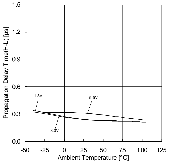
Figure 20. 立ち下がり伝播遅延(H-L)-温度特性 (R L =10kΩ, V RL =3V, C L =15pF I N =-1.5V, 100mV Overdrive)
