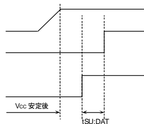
Figure 54. SCL='H' SDA='L'の時
