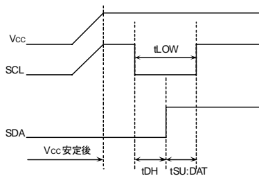
Figure 53. SCL='H' SDA='L'の時
