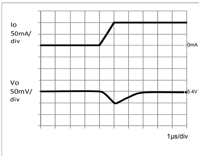
Figure 4. Transient Response (Io = 0A→0.1A) (C OUT = 1μF)
