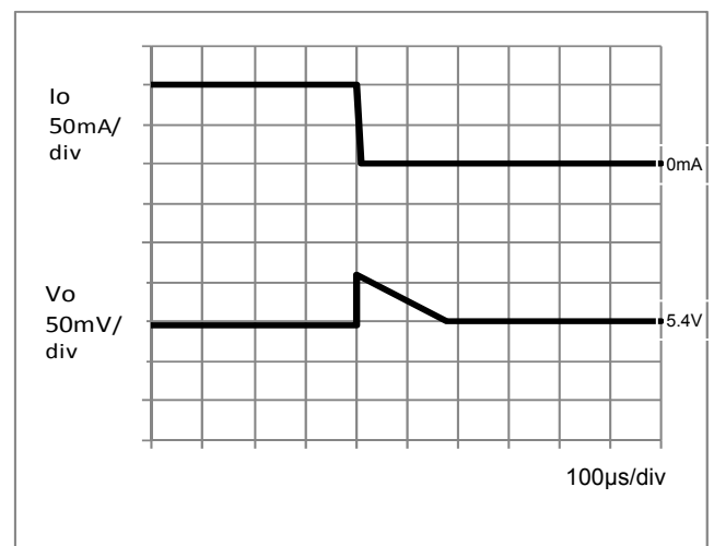
Figure 5. Transient Response (Io = 0.1A→0A) (C OUT = 1μF)
