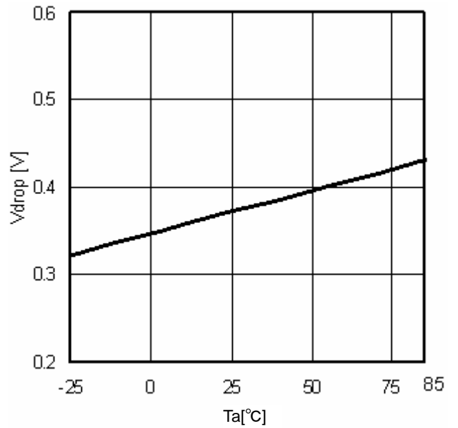
Fig.18 Minimum dropout Voltage ( V_{cc}=5V, I_o=0.3A )
