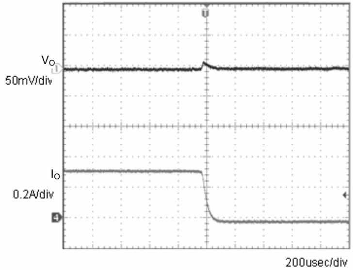
Fig.4 Transient Response (0.3→0A) C_o=1\mu\text{F}
