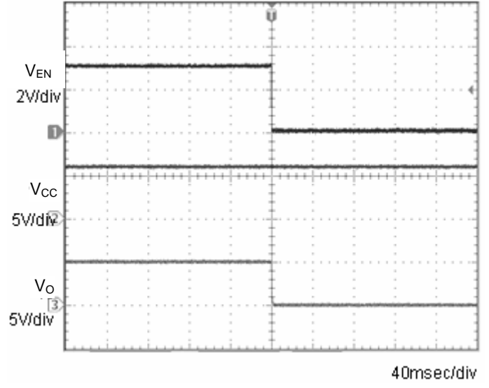
Fig.8 OFF sequence 2 Co=1μF
