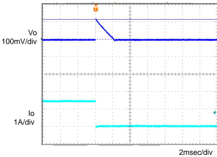
Figure 7. Transient Response (1.5→0A) Co=1μF, Ta=25°C
