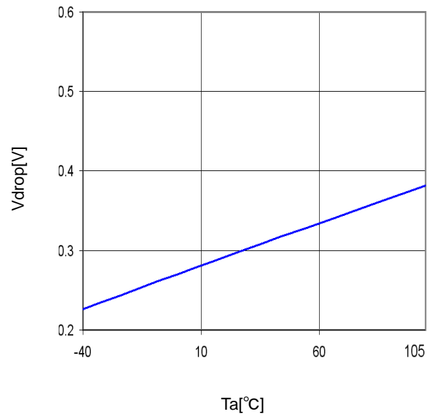
Figure 30. Minimum dropout Voltage1 (Vcc=6V, Io=1.0A)
