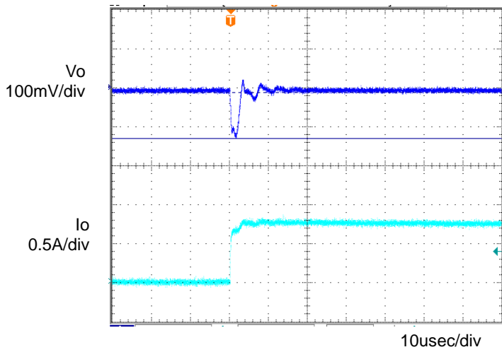
Figure 3. Transient Response (0→1.5A) Co=1μF, Ta=-40°C
