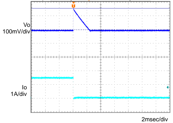
Figure 8. Transient Response (1.5→0A) Co=1μF, Ta=105°C
