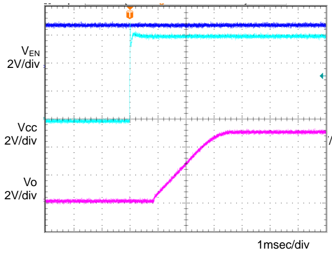
Figure 11. Input sequence 1 C_o=1\mu F, T_a=105^\circ C
