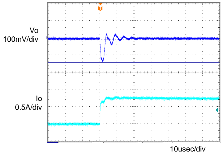
Figure 4. Transient Response (1.5→0A) Co=1μF, Ta=25°C
