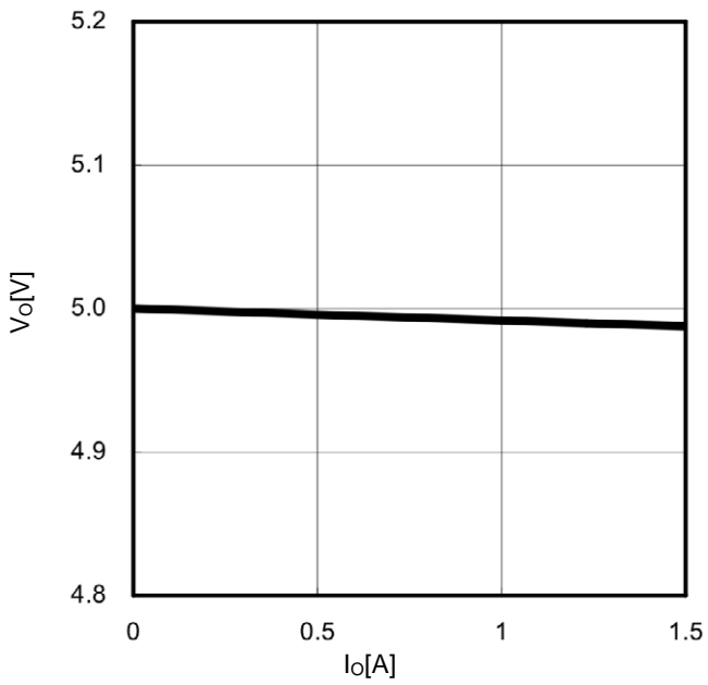
Figure 25. Io-Vo
