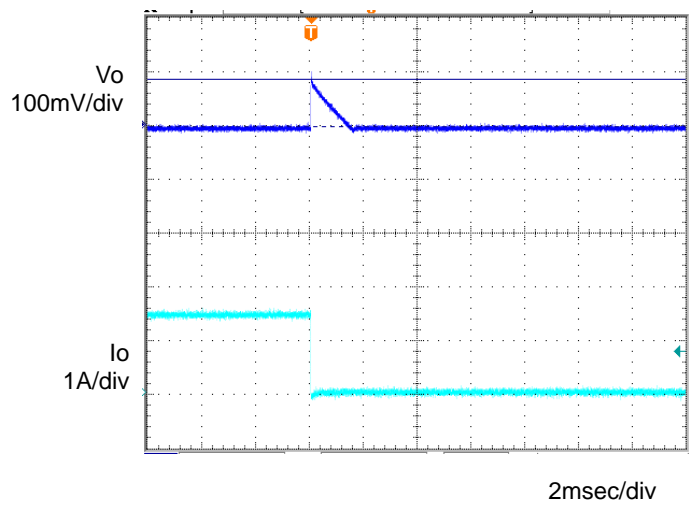
Figure 6. Transient Response (1.5→0A) Co=1μF, Ta=-40°C
