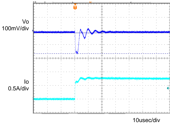
Figure 5. Transient Response (0→1.5A) Co=1μF, Ta=105°C
