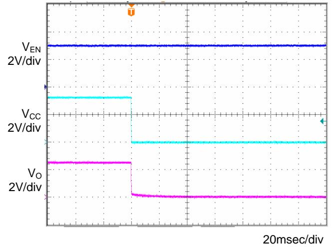
Fig.14 OFF sequence 1 C_o = 1\mu\text{F} , T_a = 105^\circ\text{C}
